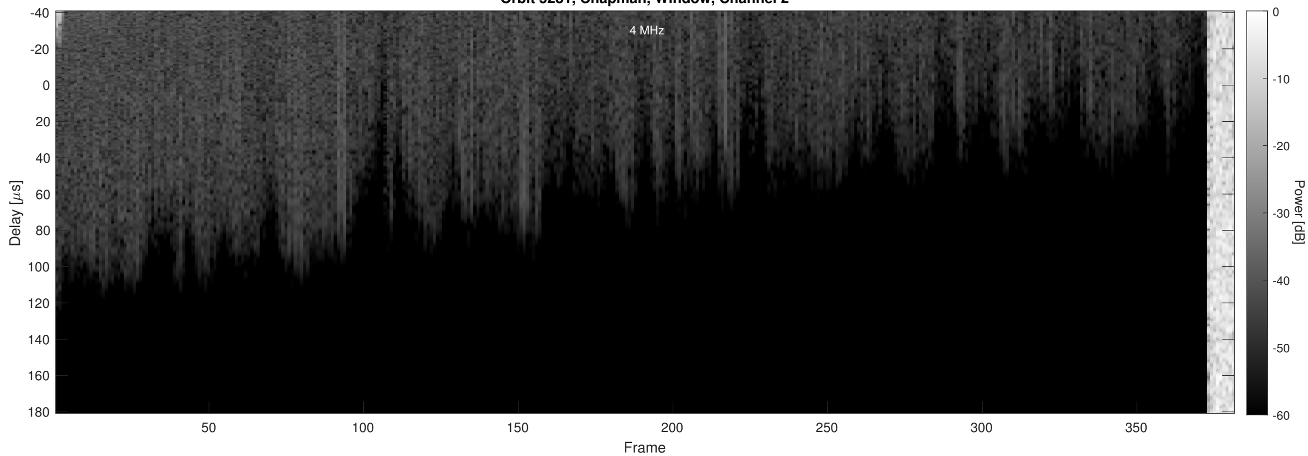
Orbit 5281, Chapman, Window, Channel 2
