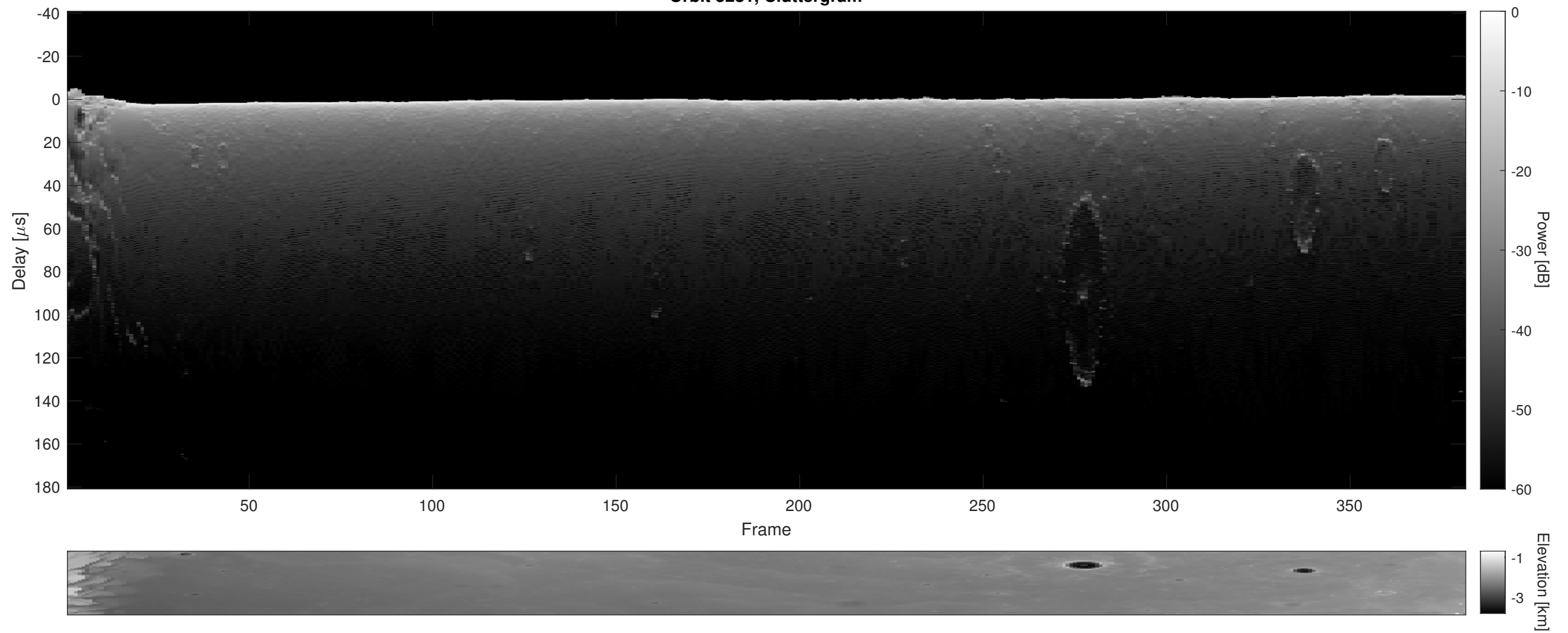
Orbit 5281, Cluttergram
