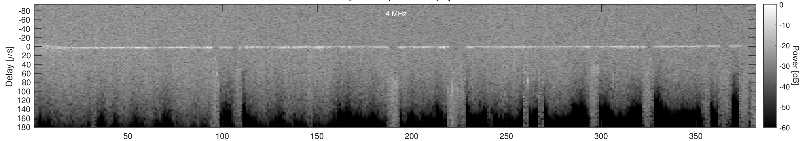
Orbit 5281, Cluttergram
