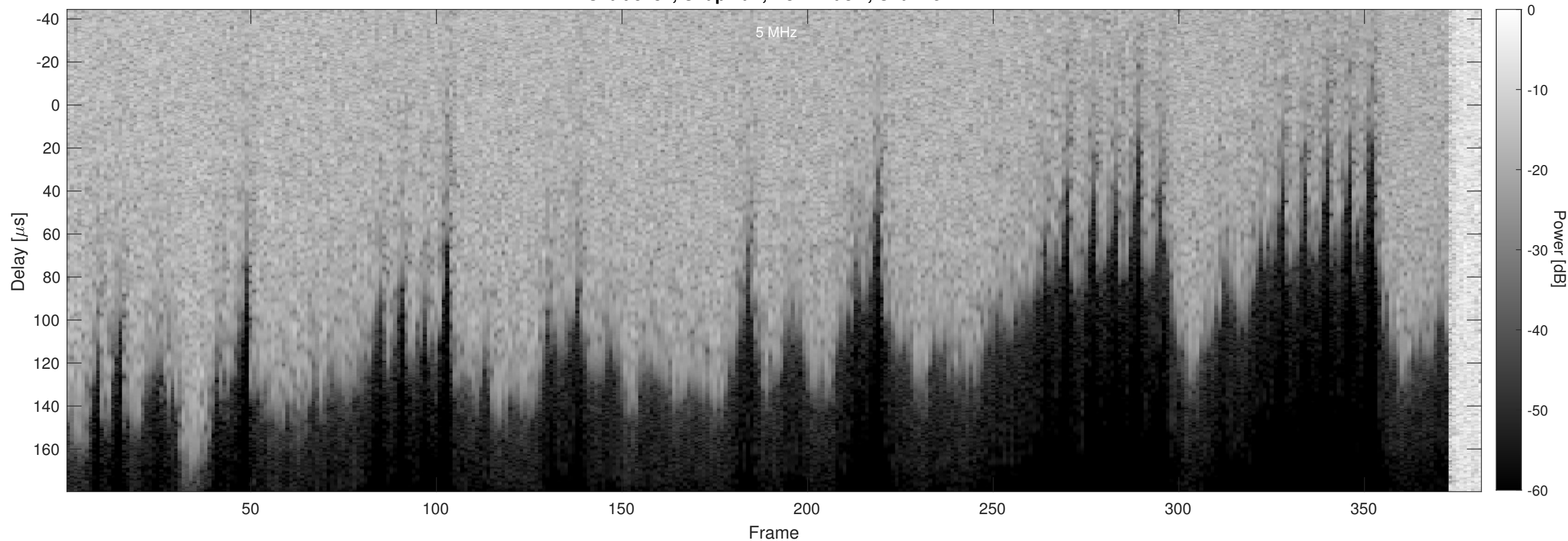
Orbit 5282, Chapman, No Window, Channel 2
