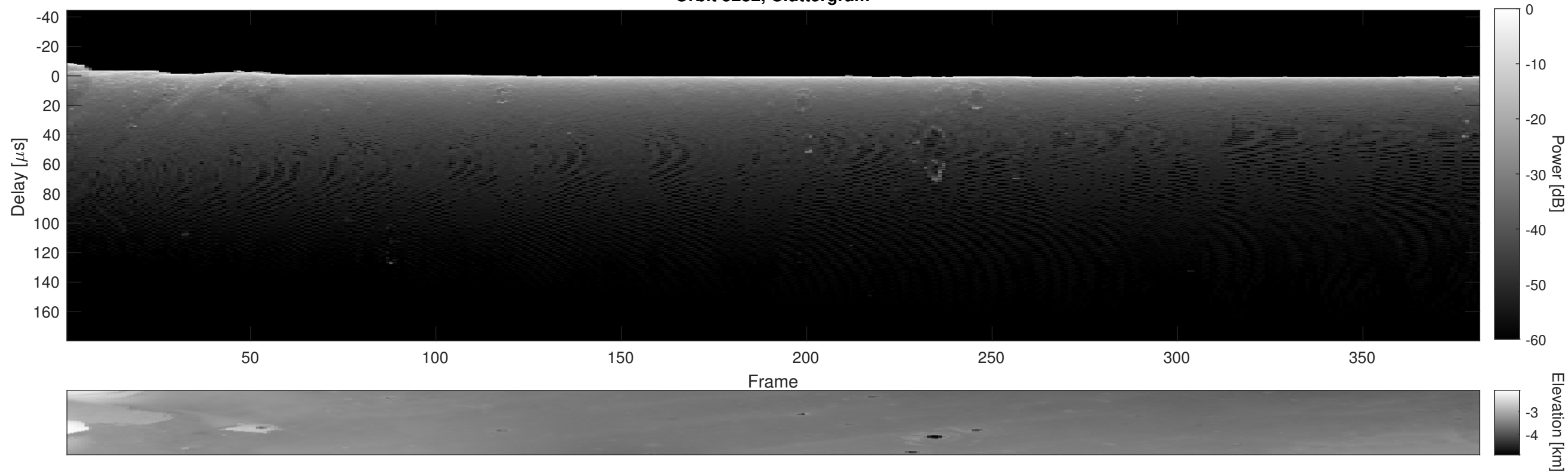
Orbit 5282, Cluttergram
