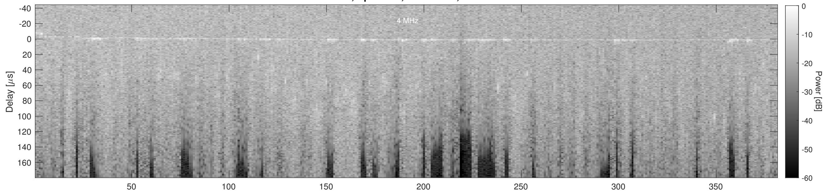
Orbit 5282, Cluttergram
