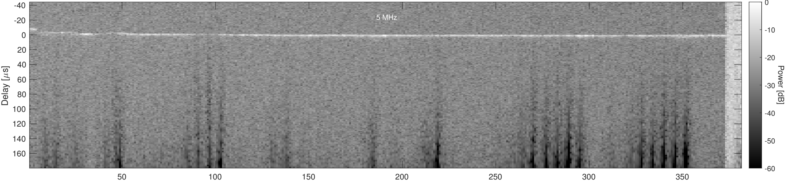
Orbit 5282, Optimized, Window, Channel 2
