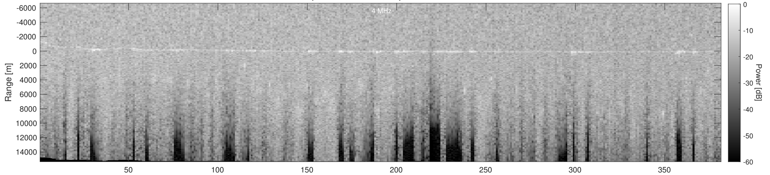
Orbit 5282, Depth-Corrected Cluttergram
