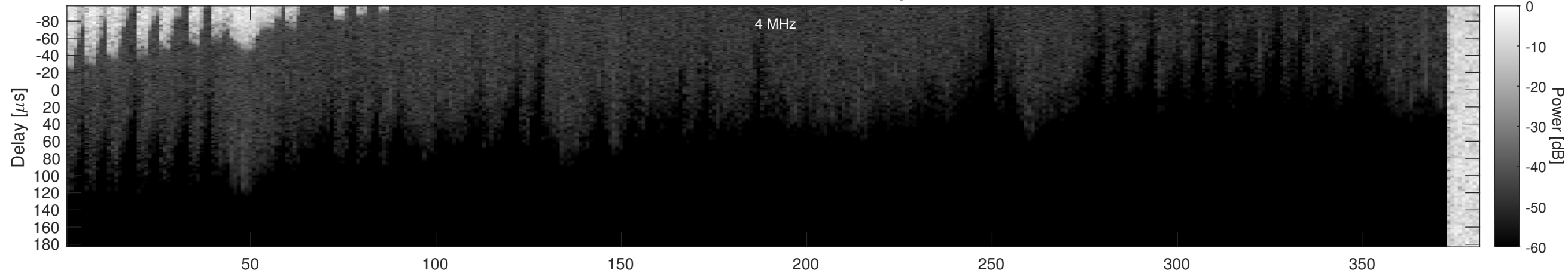
Orbit 5283, Window, Channel 2, Optimized
