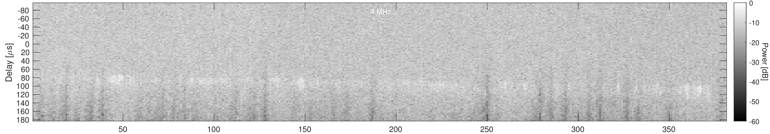
Orbit 5283, Window, Channel 2, Chapman
