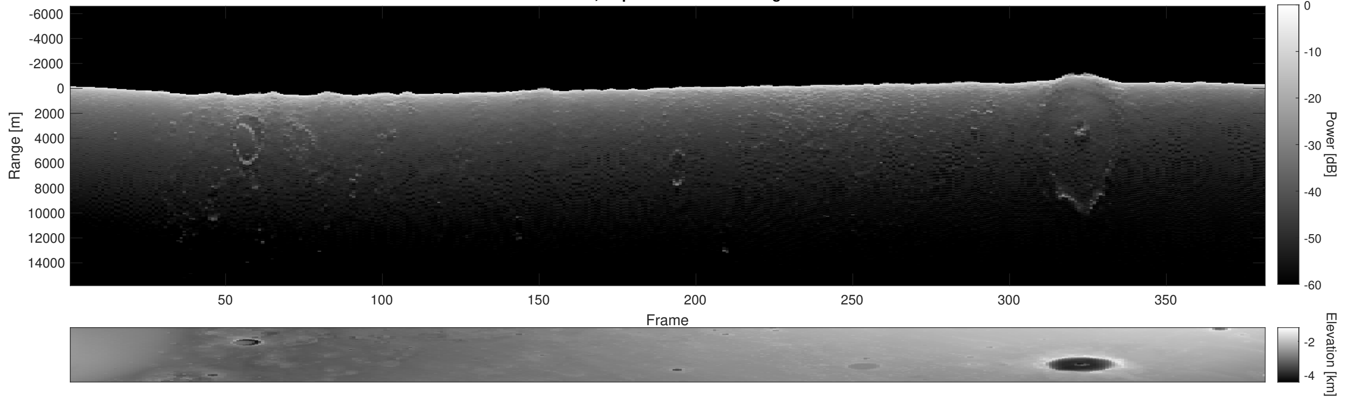
Orbit 5283, Depth-Corrected Cluttergram
