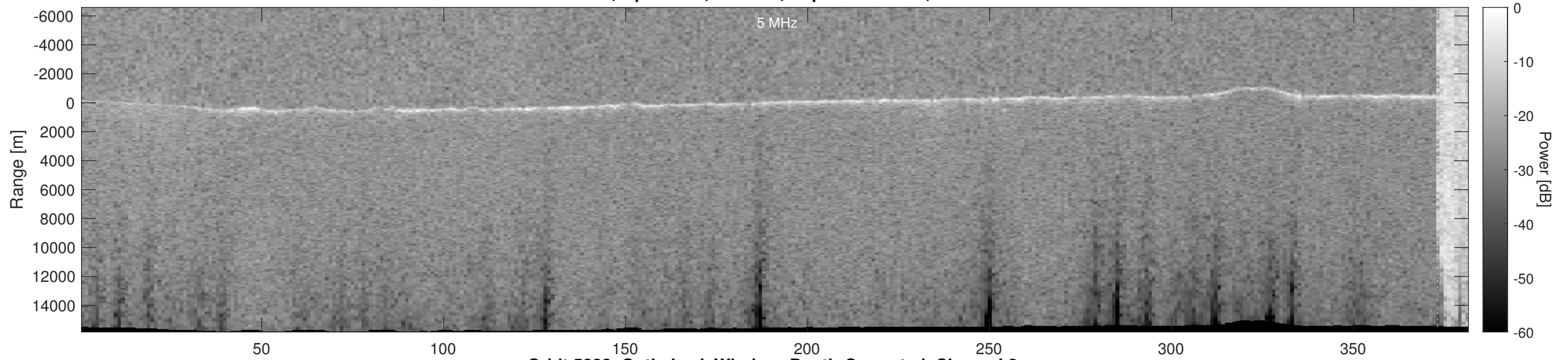
Orbit 5283, Optimized, Window, Depth-Corrected, Channel 2
