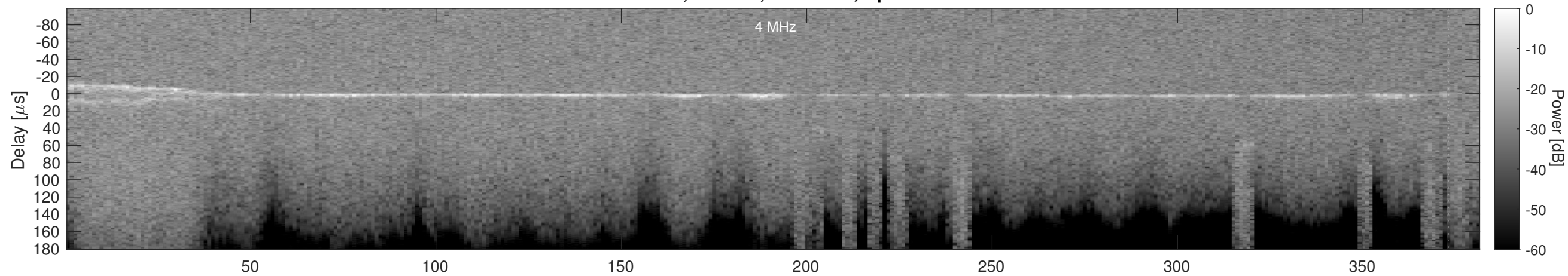
Orbit 5285, Cluttergram
