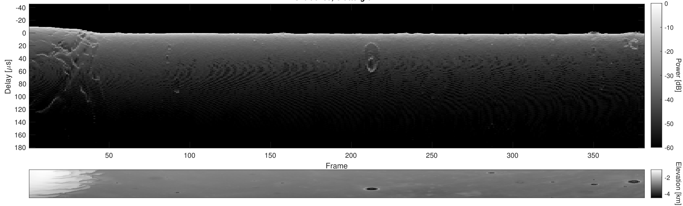
Orbit 5285, Cluttergram
