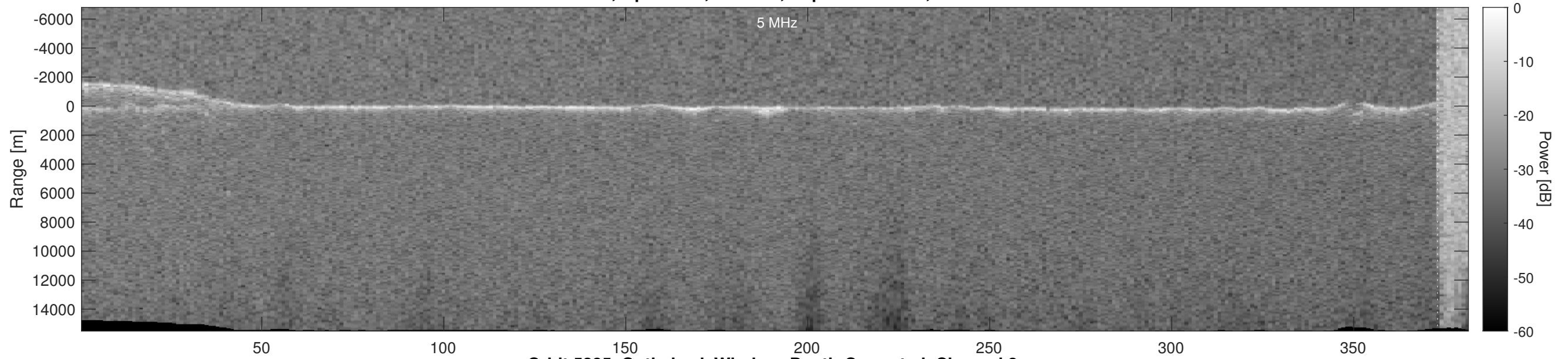
Orbit 5285, Optimized, Window, Depth-Corrected, Channel 2
