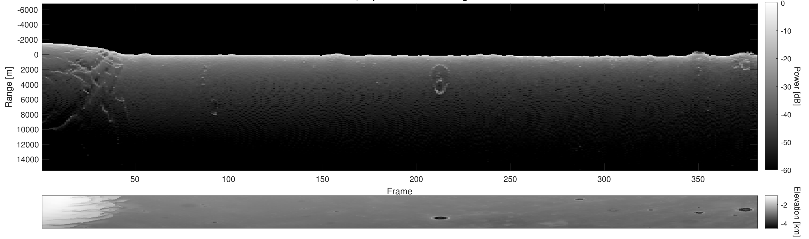
Orbit 5285, Depth-Corrected Cluttergram
