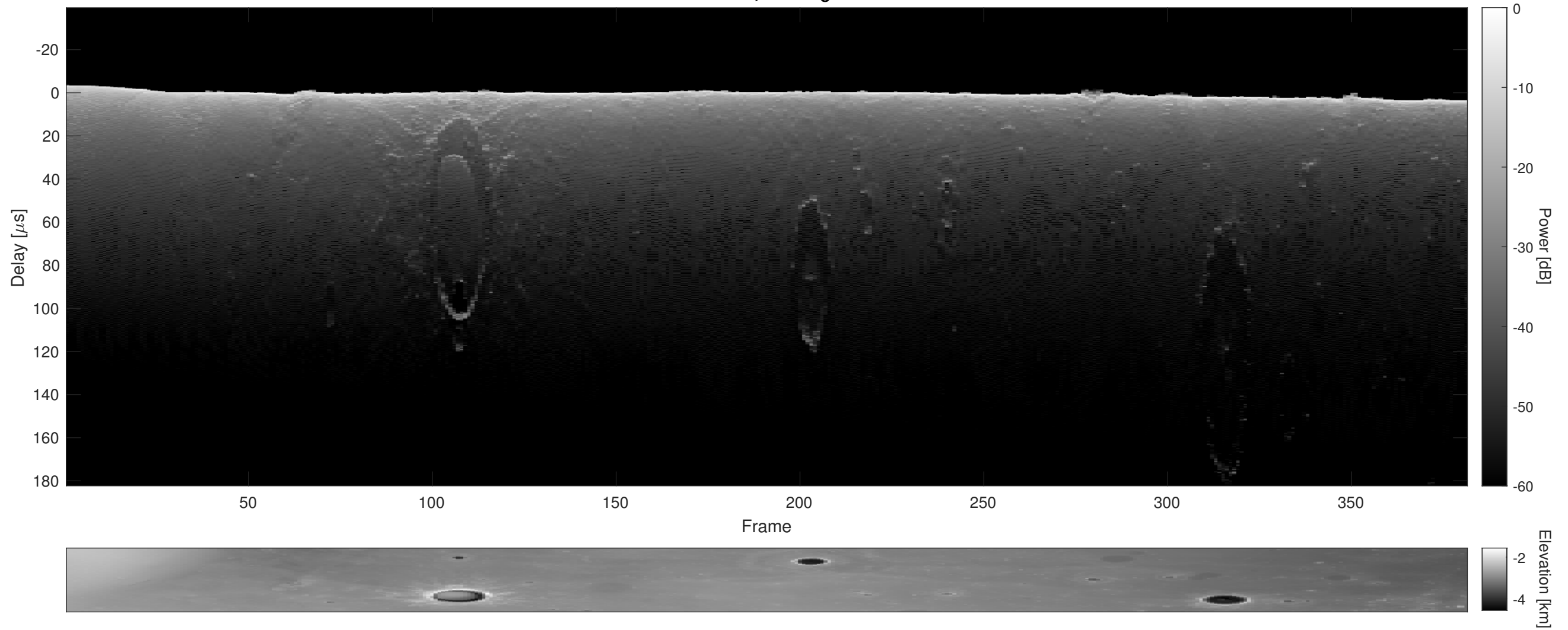
Orbit 5287, Cluttergram
