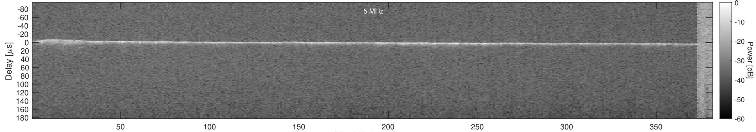
Orbit 5289, Cluttergram
