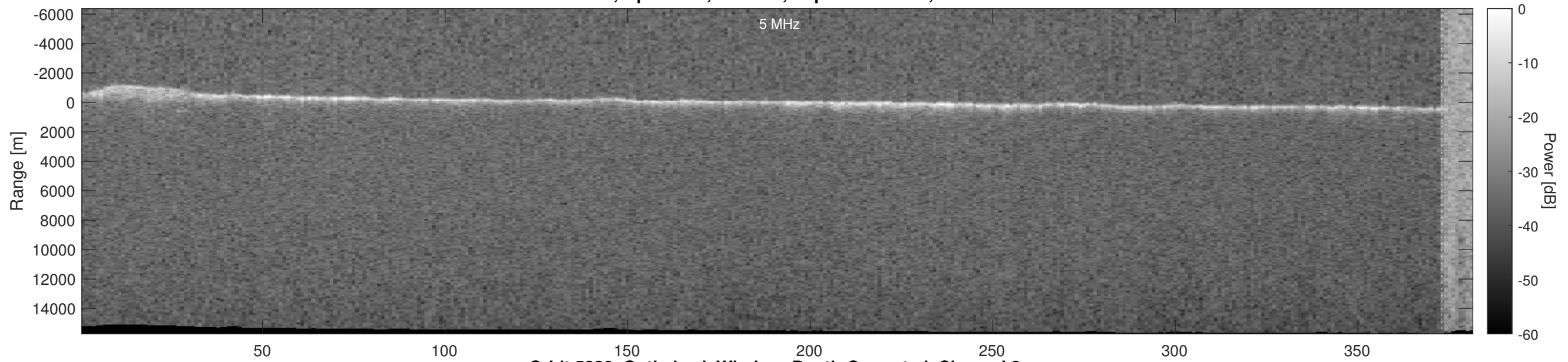
Orbit 5289, Optimized, Window, Depth-Corrected, Channel 2
