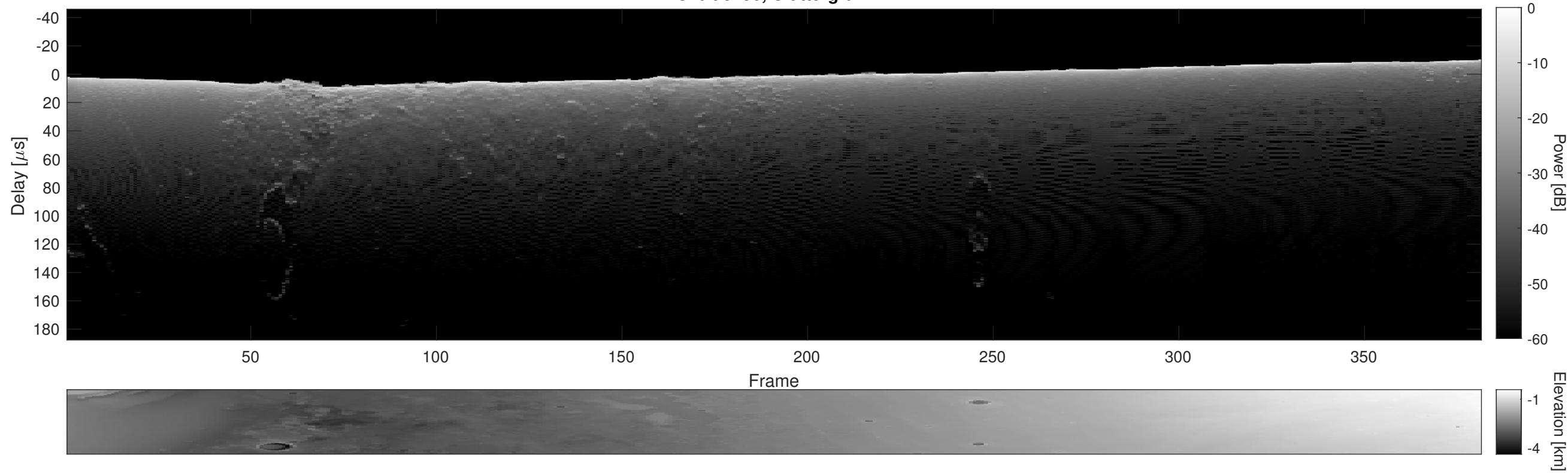
Orbit 5290, Cluttergram
