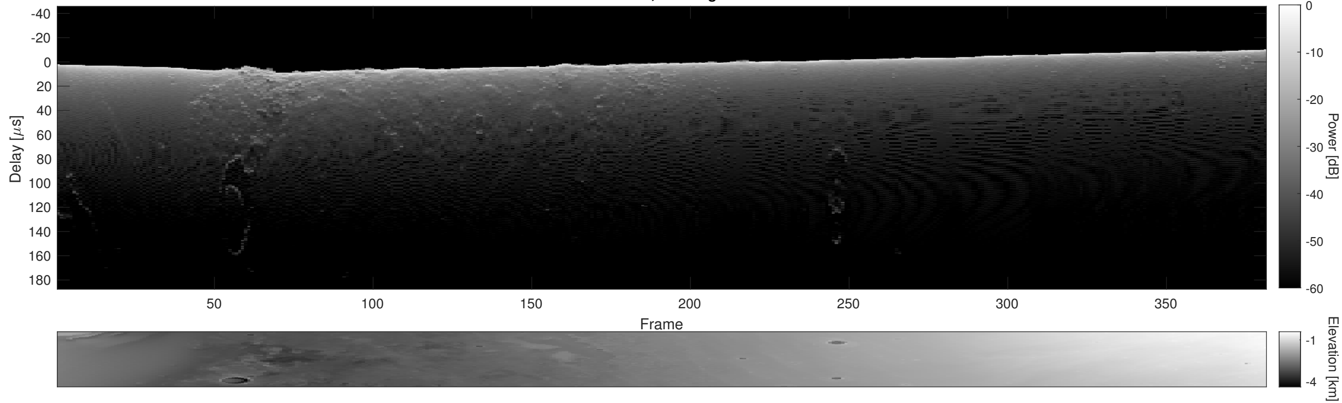
Orbit 5290, Cluttergram
