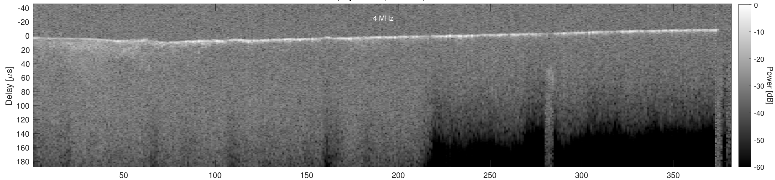
Orbit 5290, Cluttergram
