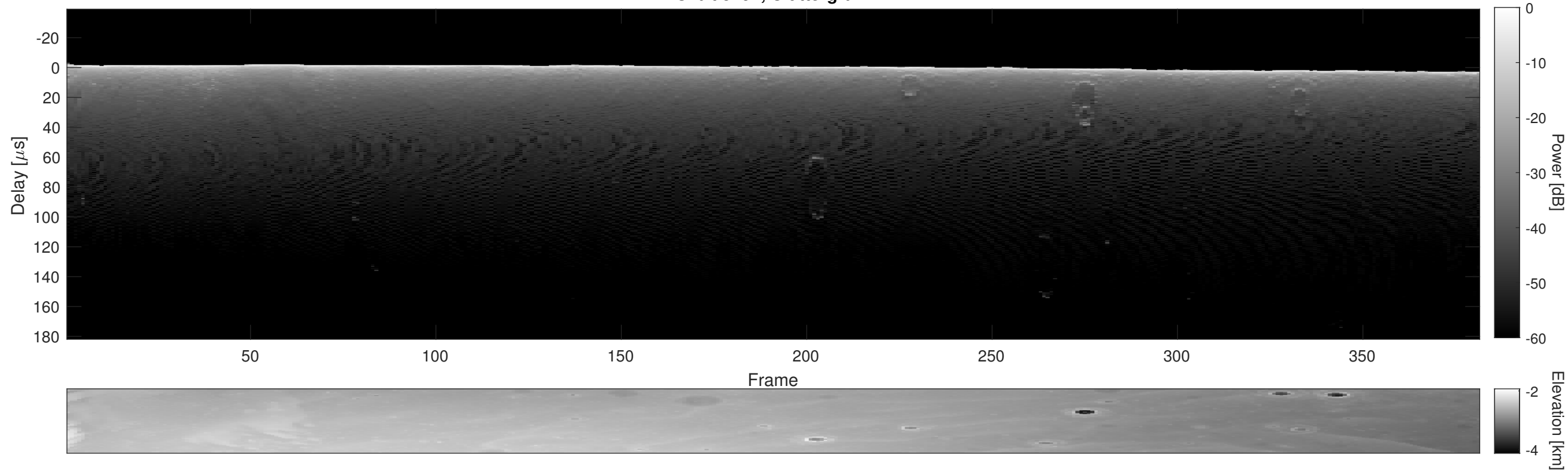
Orbit 5291, Cluttergram
