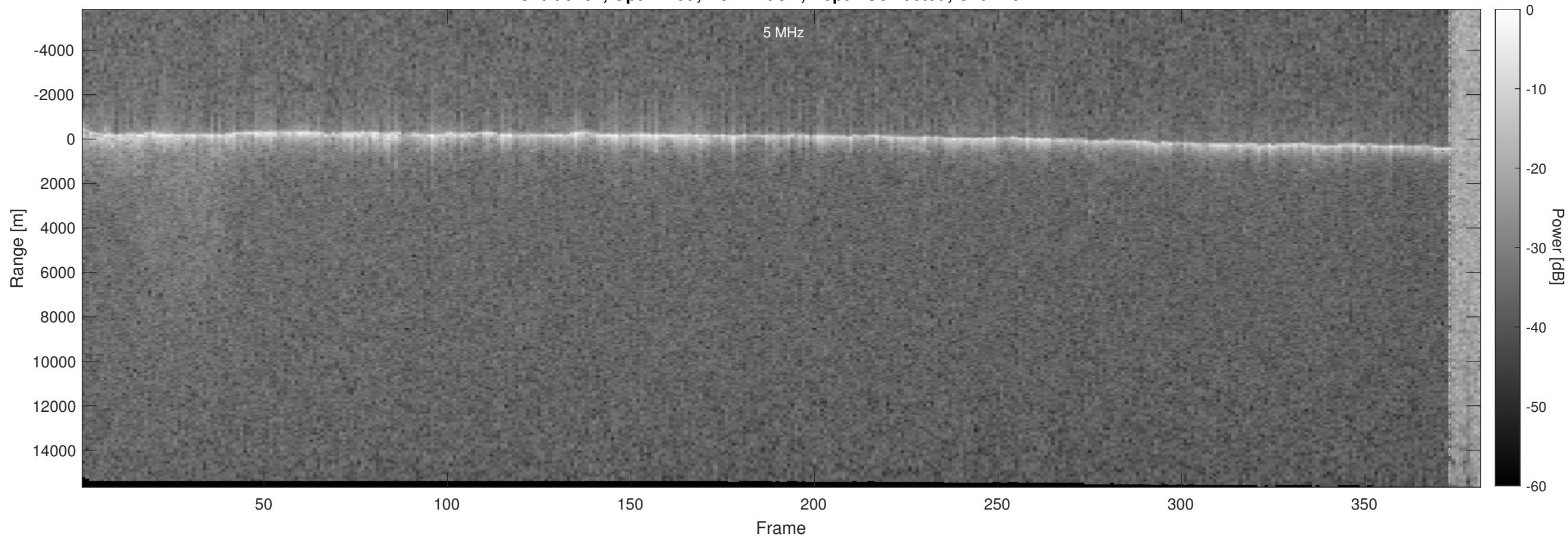
Orbit 5291, Optimized, No Window, Depth-Corrected, Channel 2
