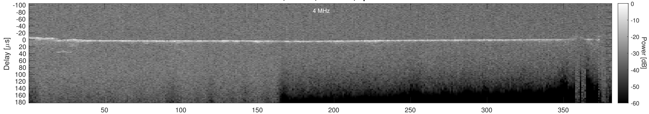
Orbit 5293, Cluttergram
