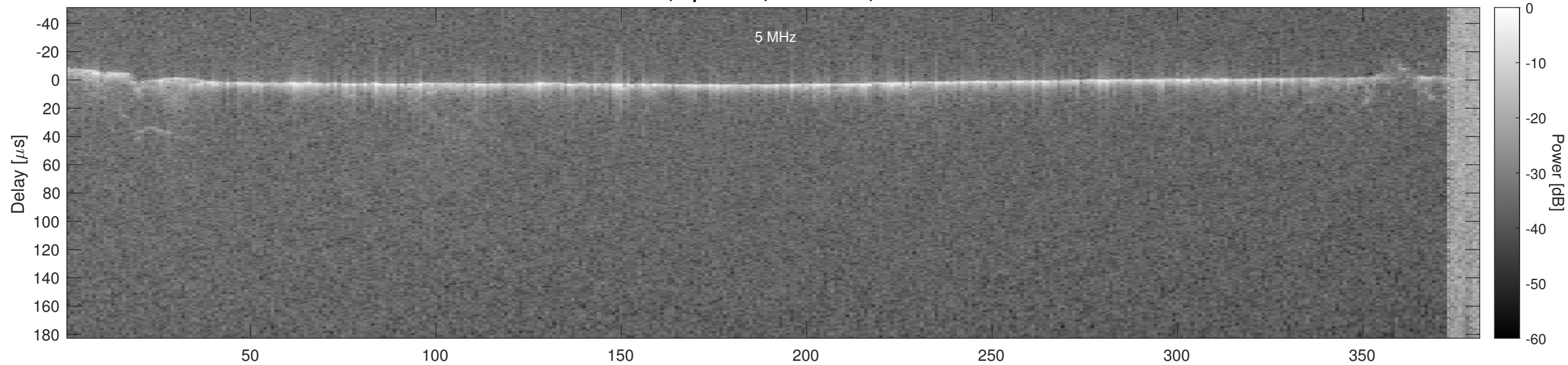
Orbit 5293, Optimized, No Window, Channel 2
