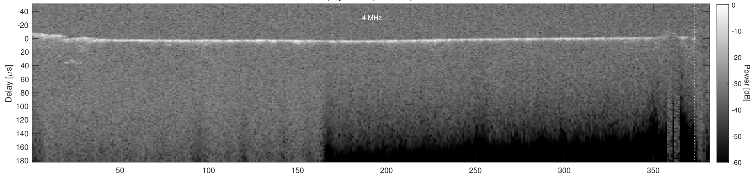
Orbit 5293, Cluttergram
