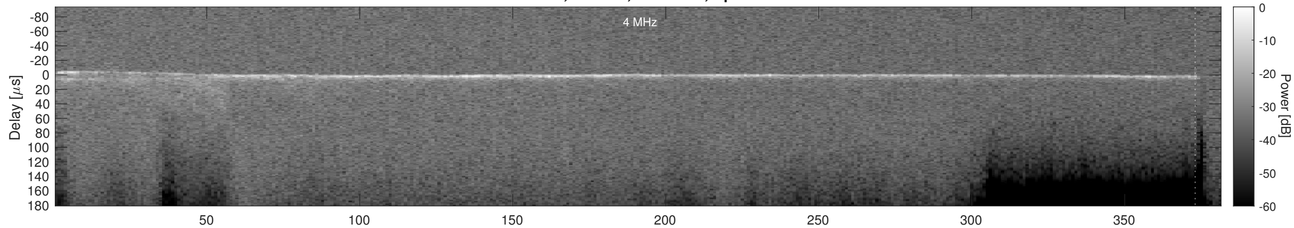
Orbit 5294, Cluttergram
