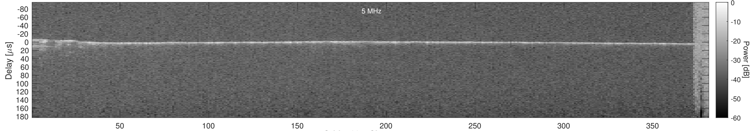
Orbit 5295, Cluttergram
