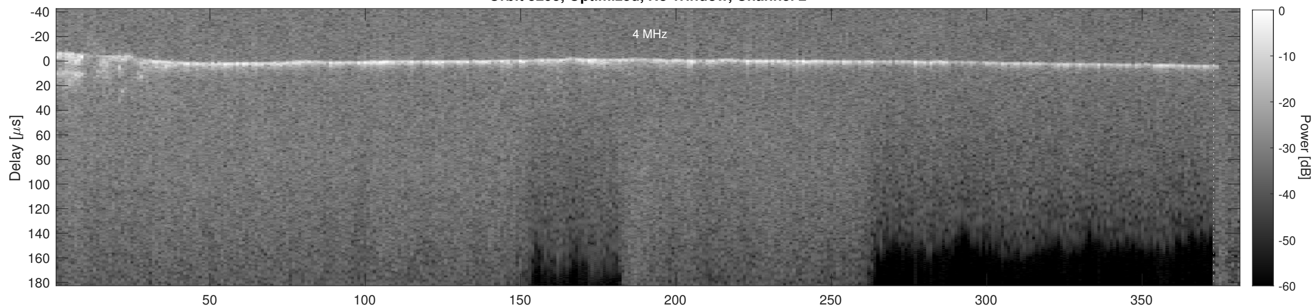
Orbit 5295, Cluttergram
