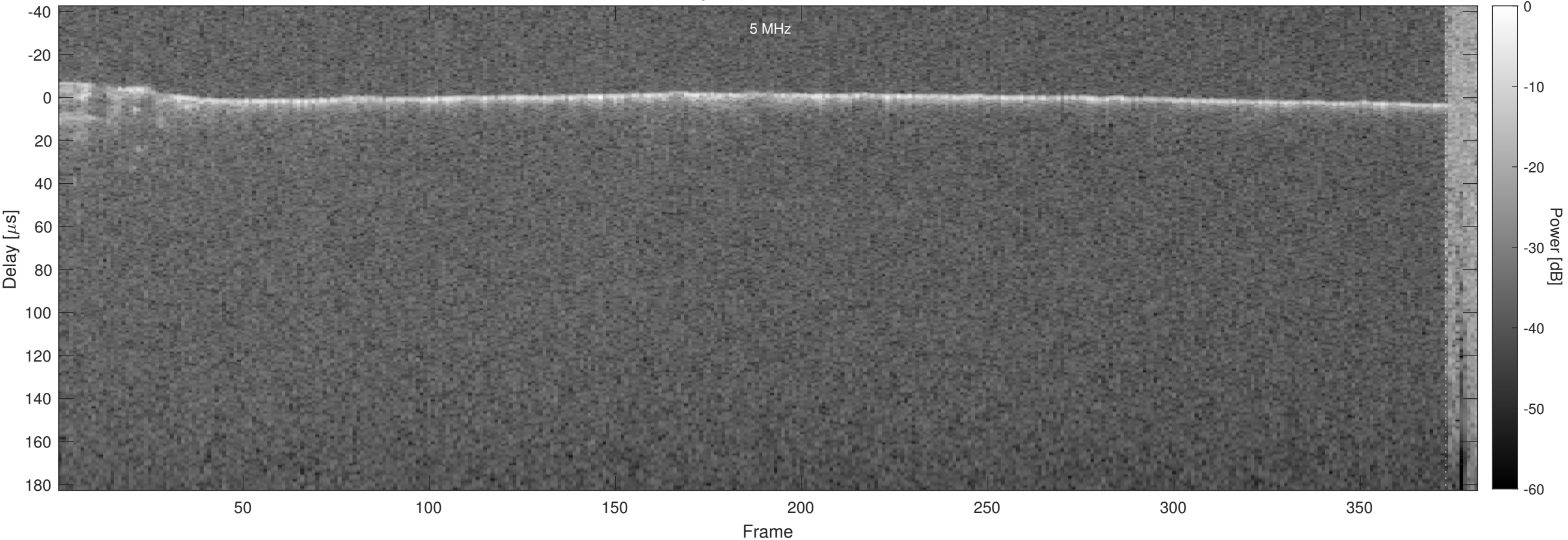
Orbit 5295, Optimized, Window, Channel 2
