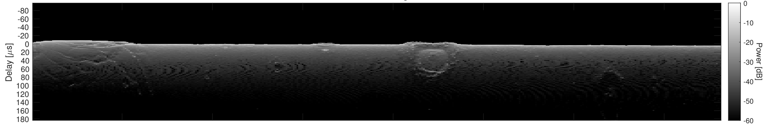
Orbit 5296, Cluttergram
