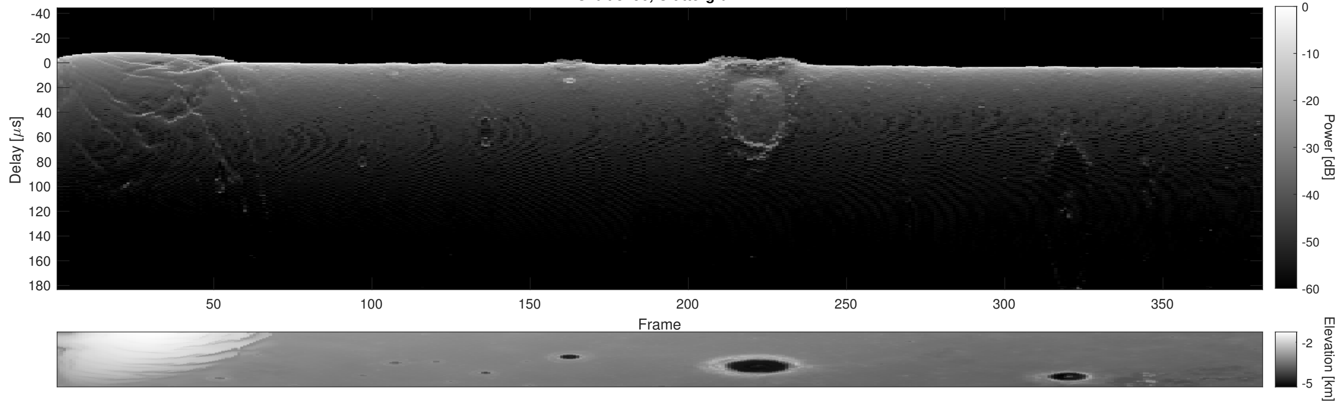
Orbit 5296, Cluttergram
