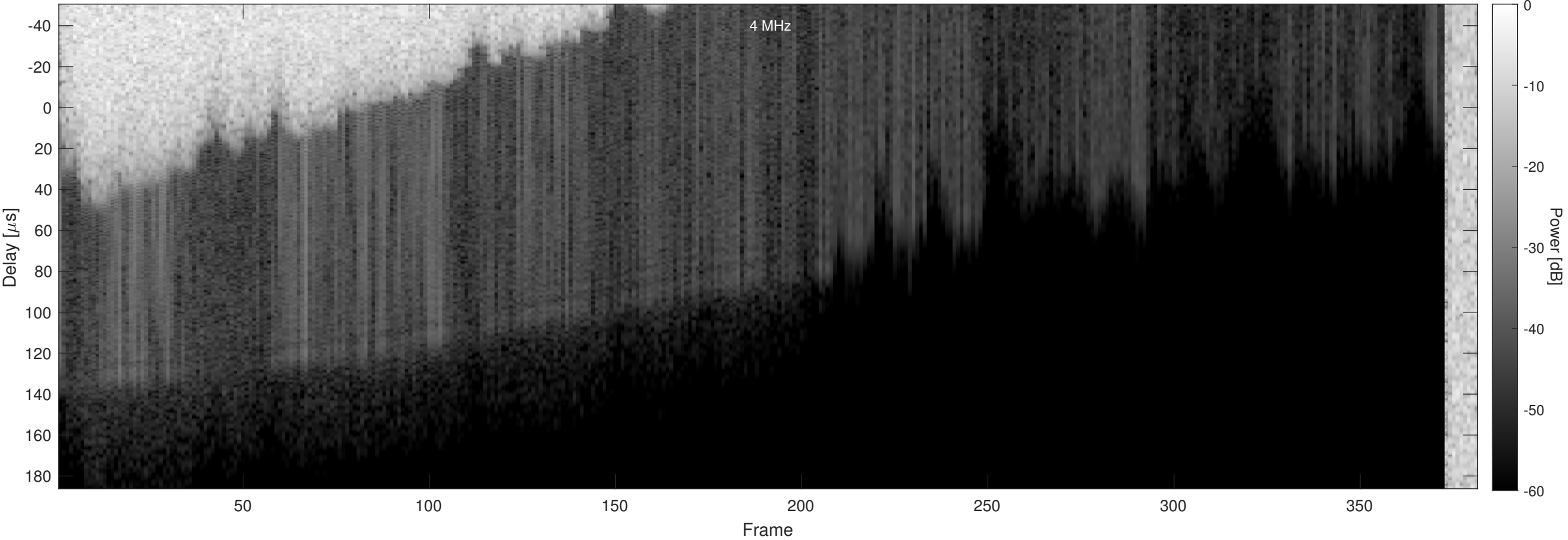
Orbit 5297, Chapman, Window, Channel 2
