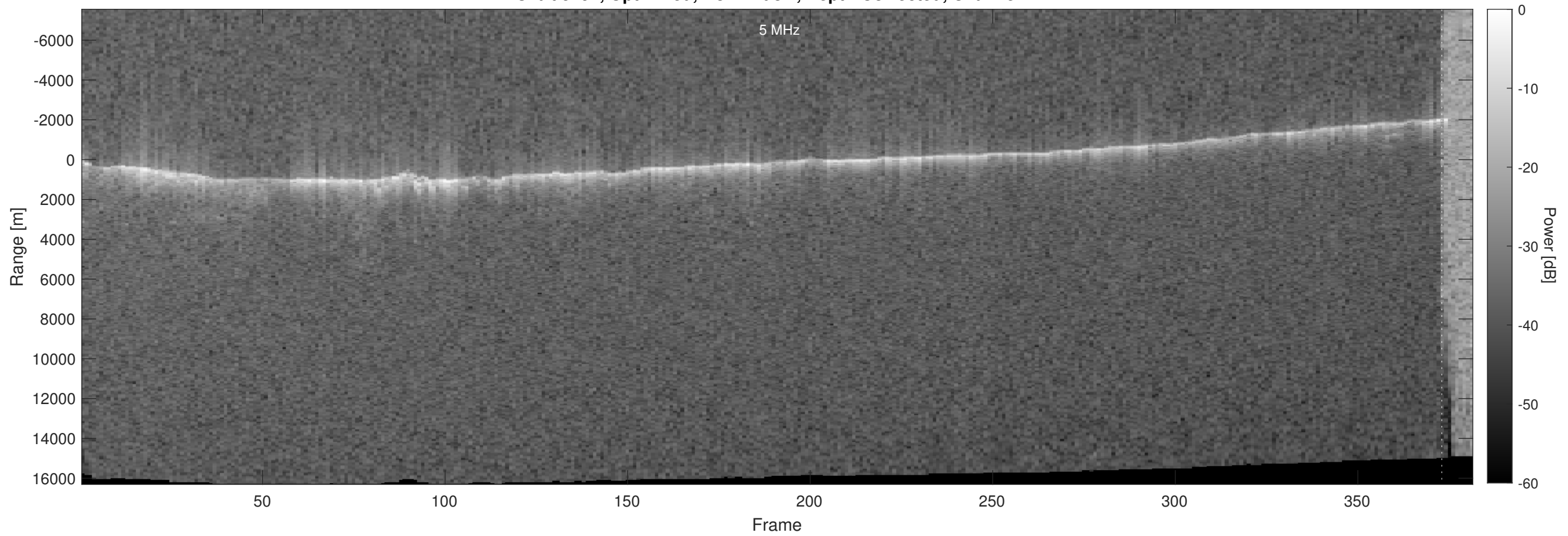
Orbit 5297, Optimized, No Window, Depth-Corrected, Channel 2
