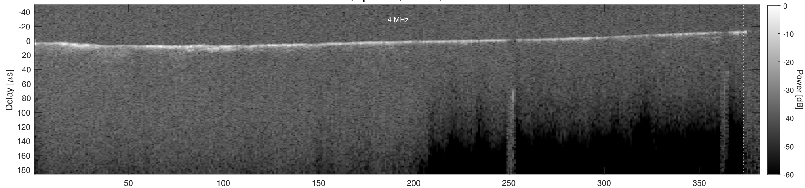
Orbit 5297, Cluttergram
