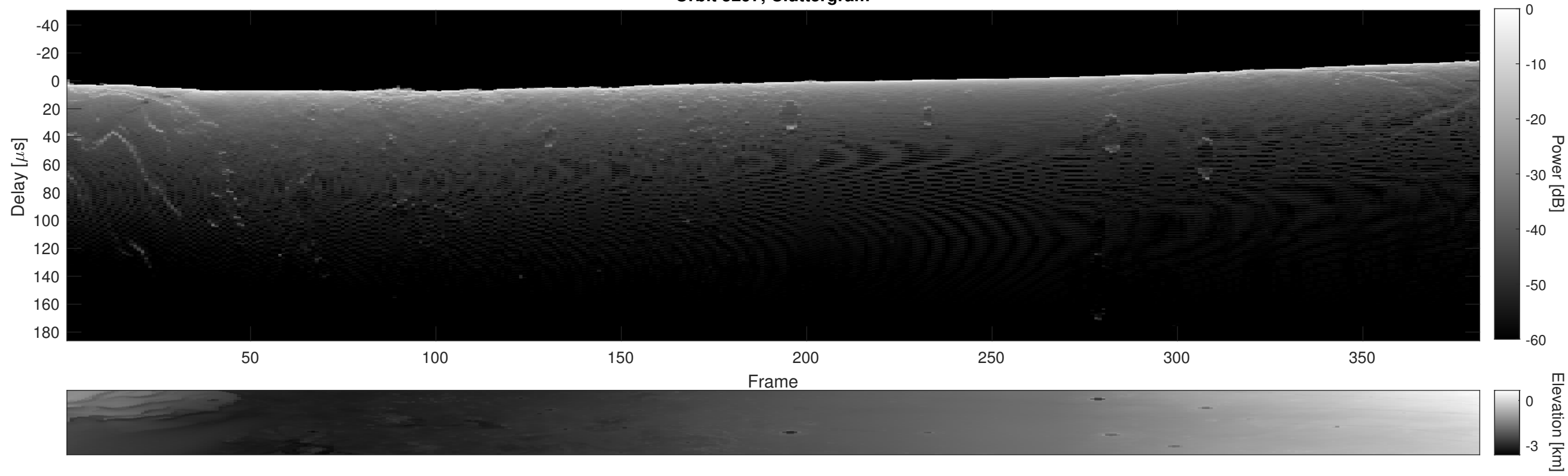
Orbit 5297, Cluttergram
