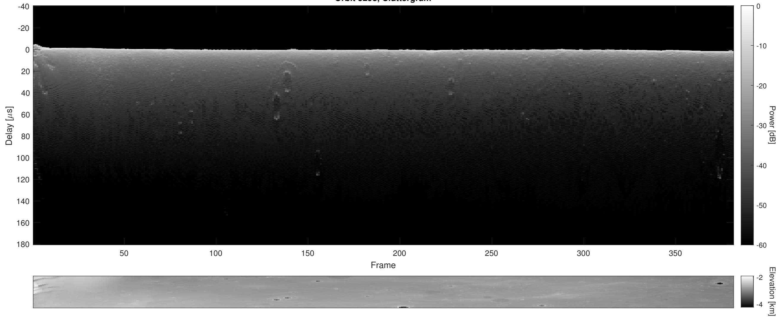
Orbit 5298, Cluttergram
