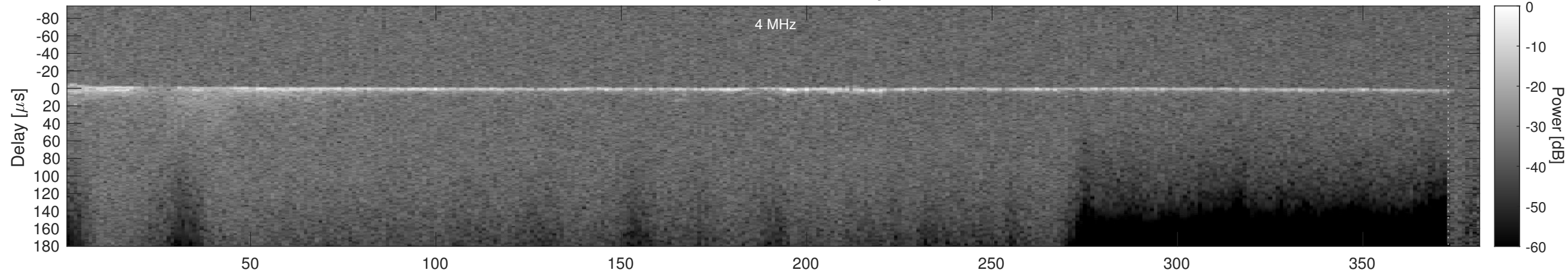
Orbit 5298, Cluttergram
