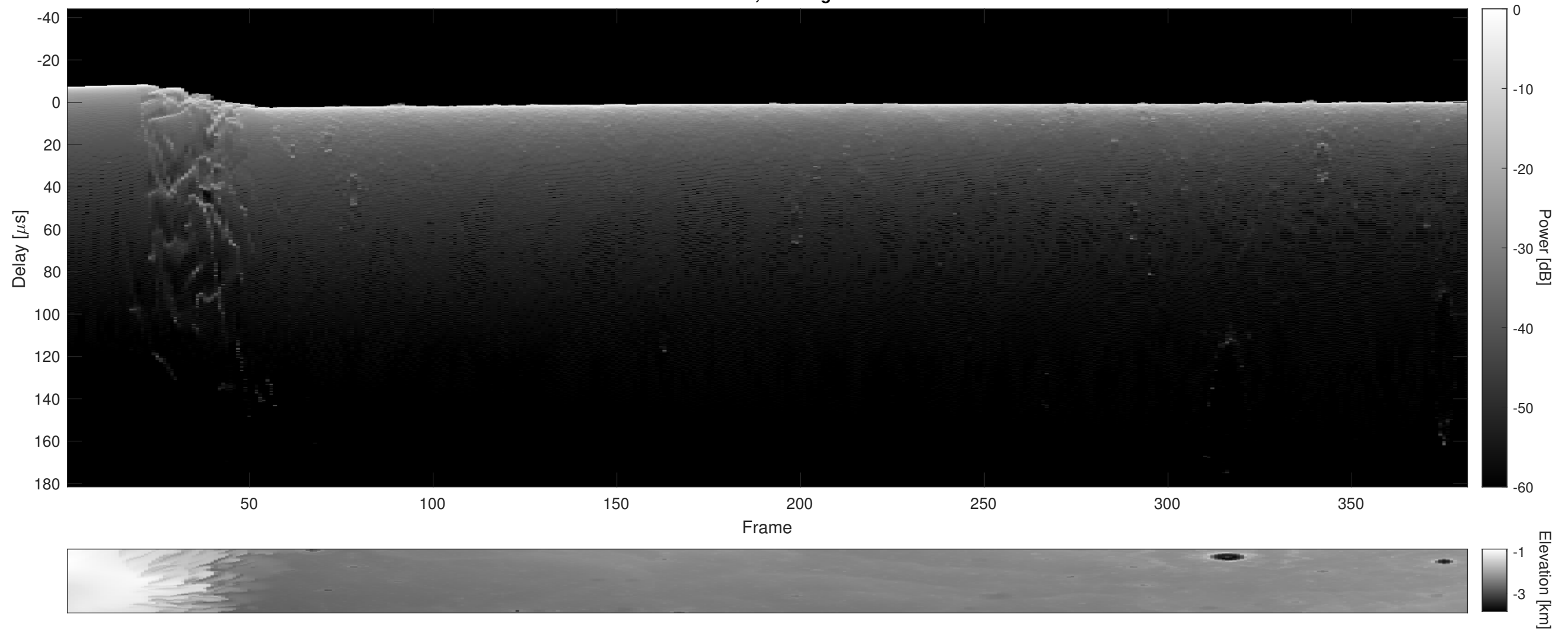
Orbit 5299, Cluttergram
