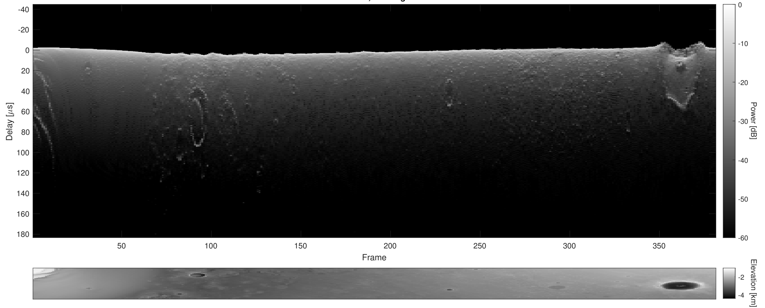
Orbit 5301, Cluttergram
