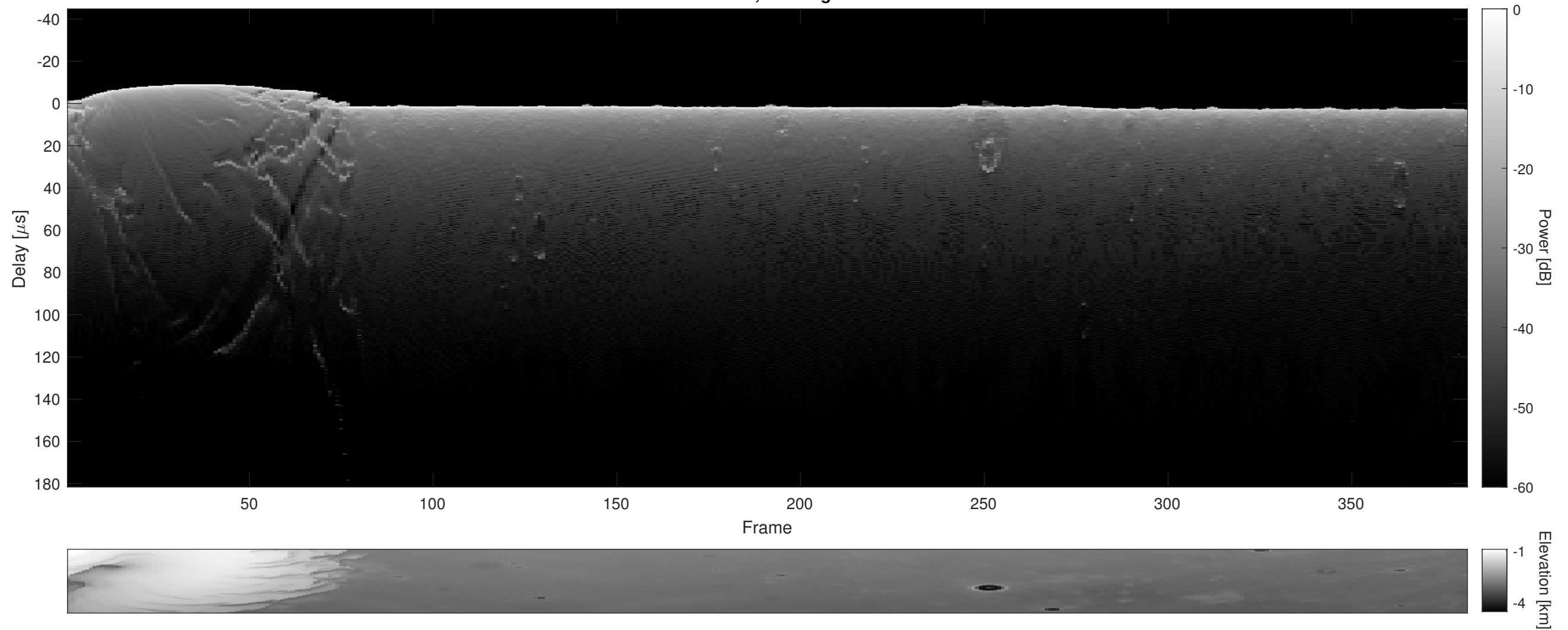
Orbit 5303, Cluttergram
