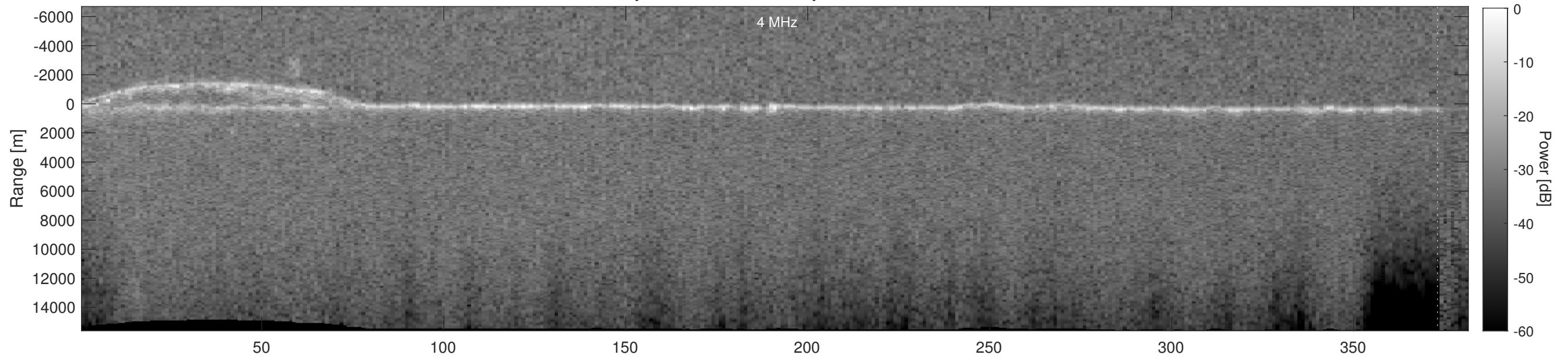
Orbit 5303, Depth-Corrected Cluttergram
