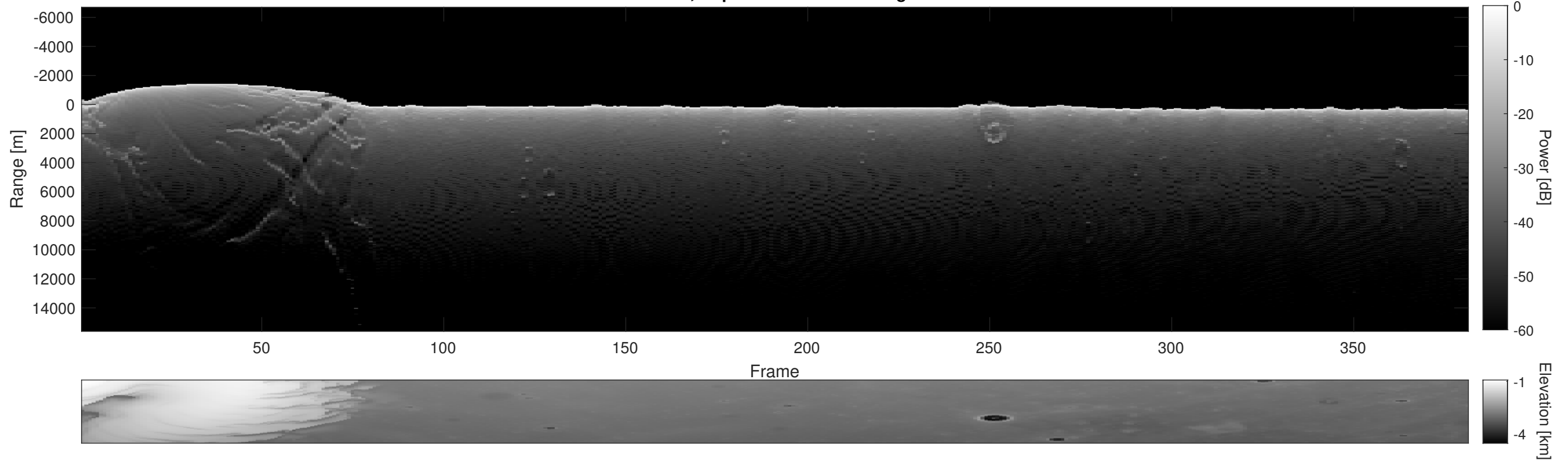
Orbit 5303, Depth-Corrected Cluttergram
