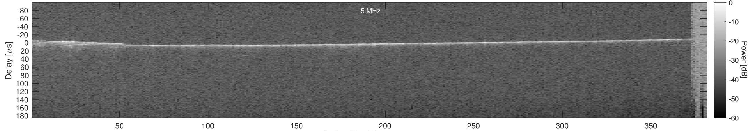
Orbit 5304, Cluttergram
