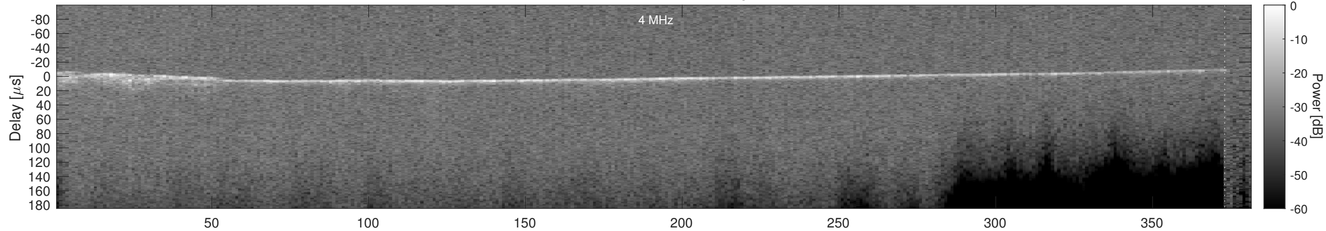
Orbit 5304, Cluttergram
