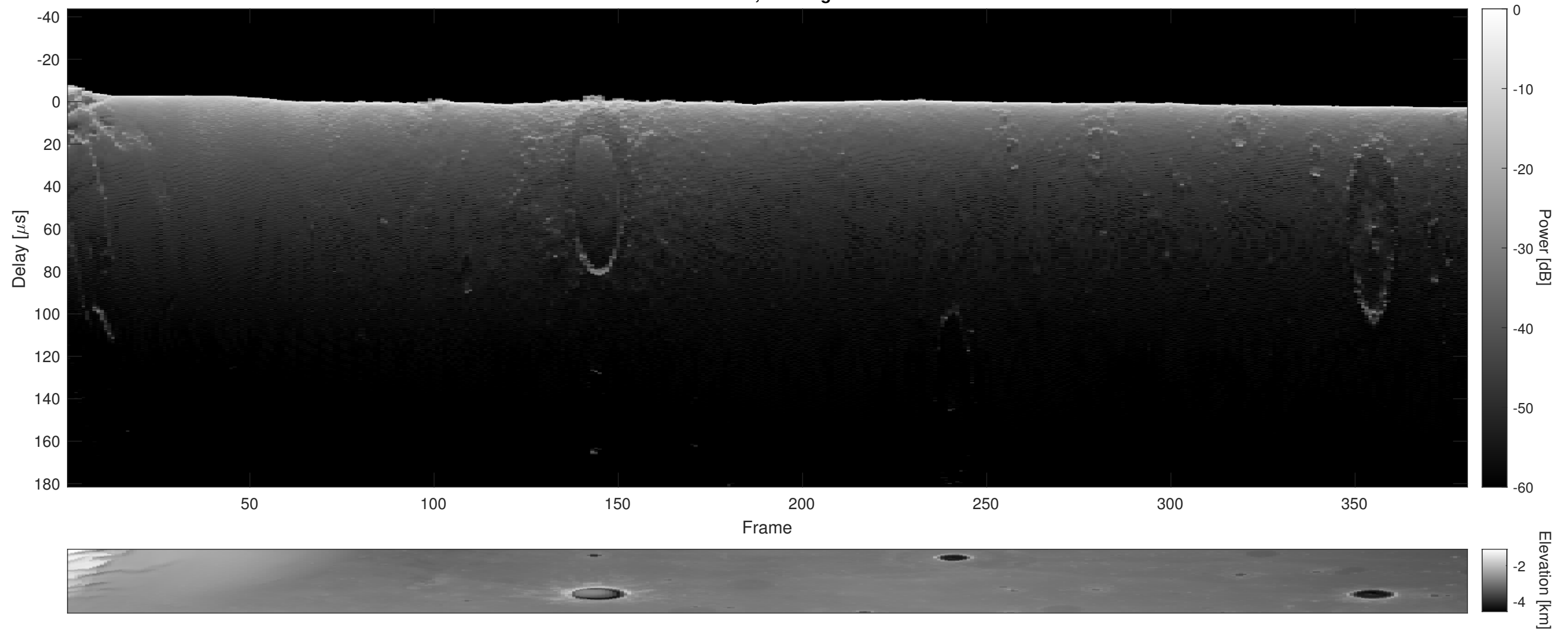
Orbit 5305, Cluttergram
