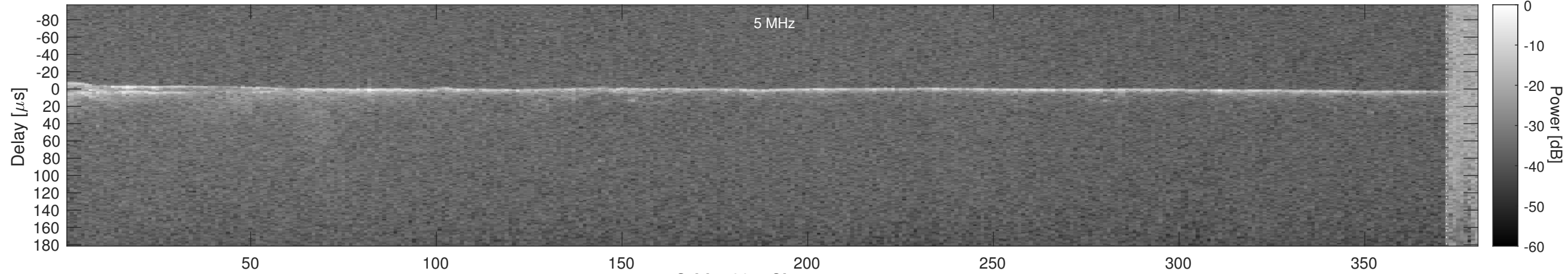
Orbit 5305, Cluttergram
