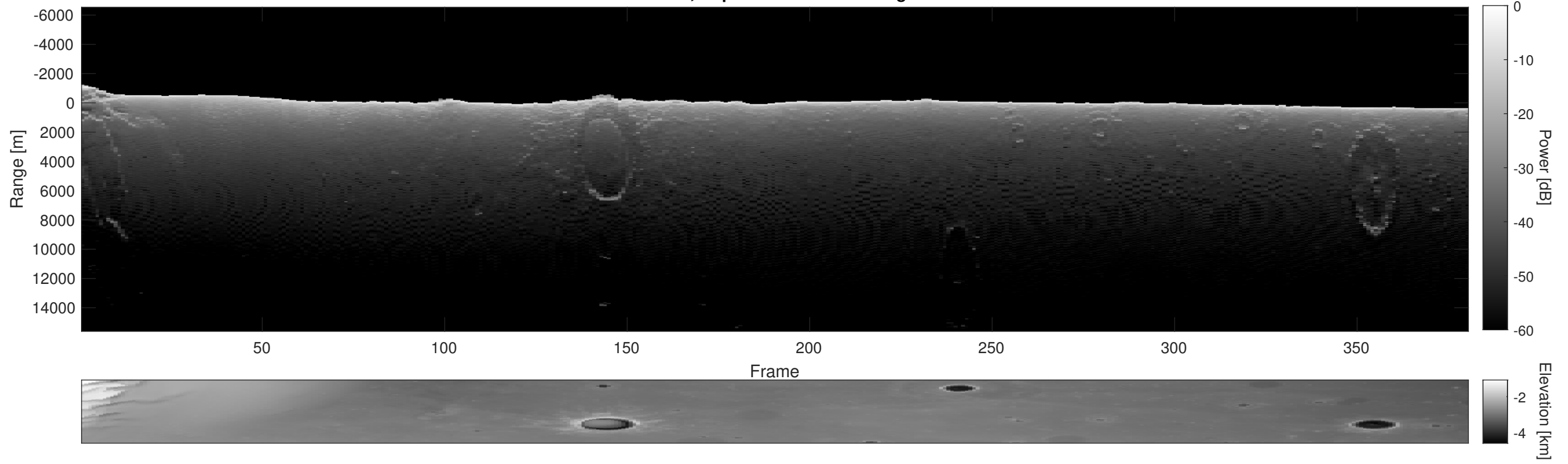
Orbit 5305, Depth-Corrected Cluttergram
