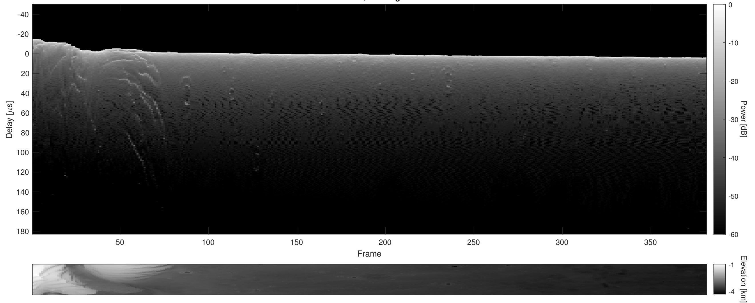
Orbit 5307, Cluttergram
