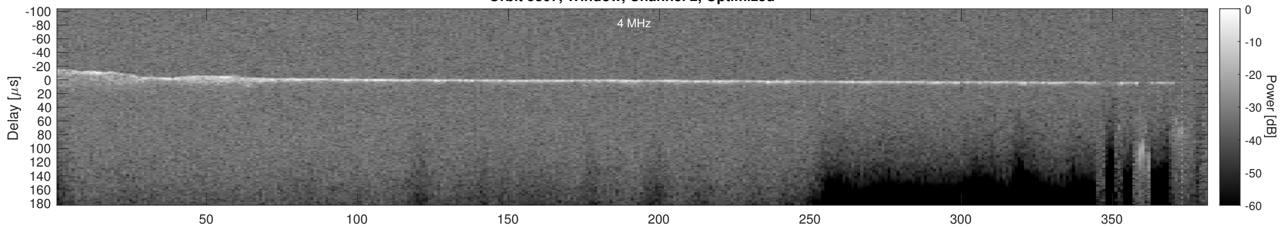
Orbit 5307, Cluttergram
