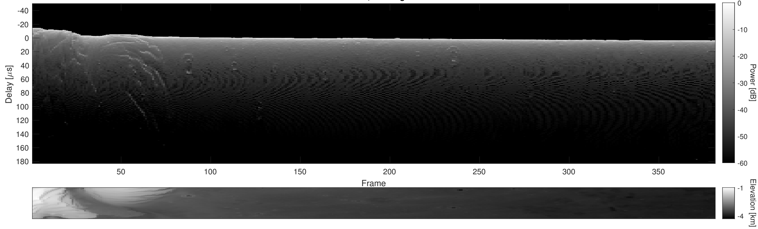
Orbit 5307, Cluttergram
