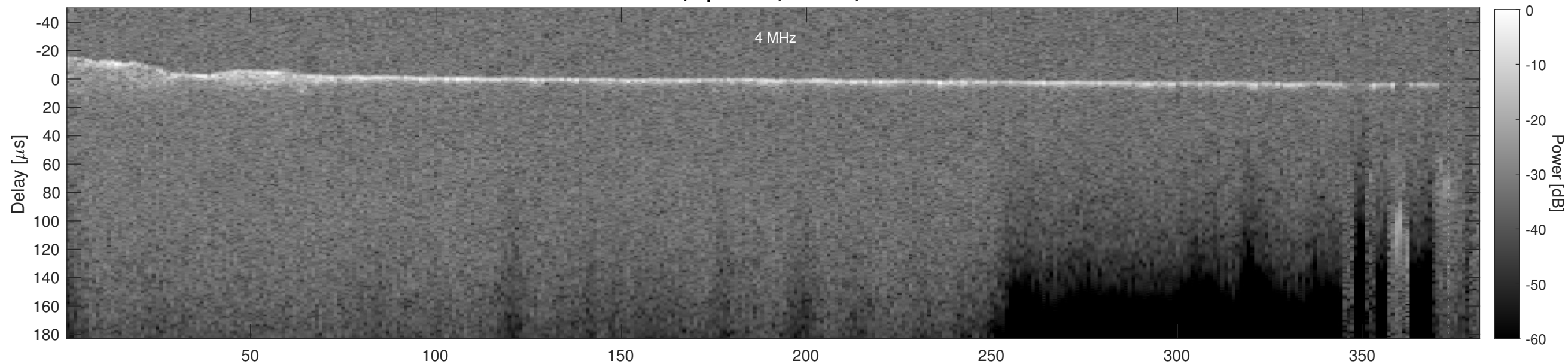
Orbit 5307, Cluttergram
