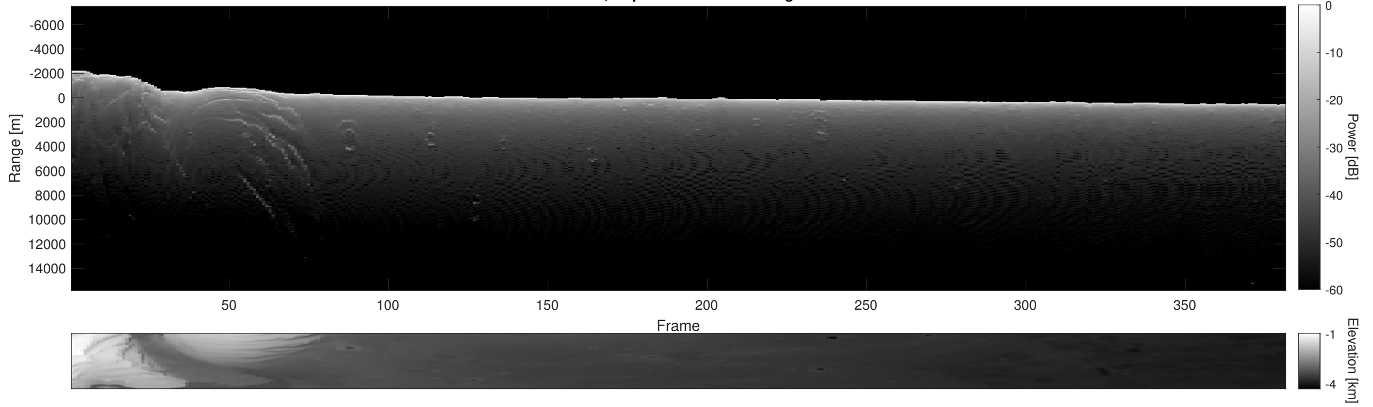
Orbit 5307, Depth-Corrected Cluttergram
