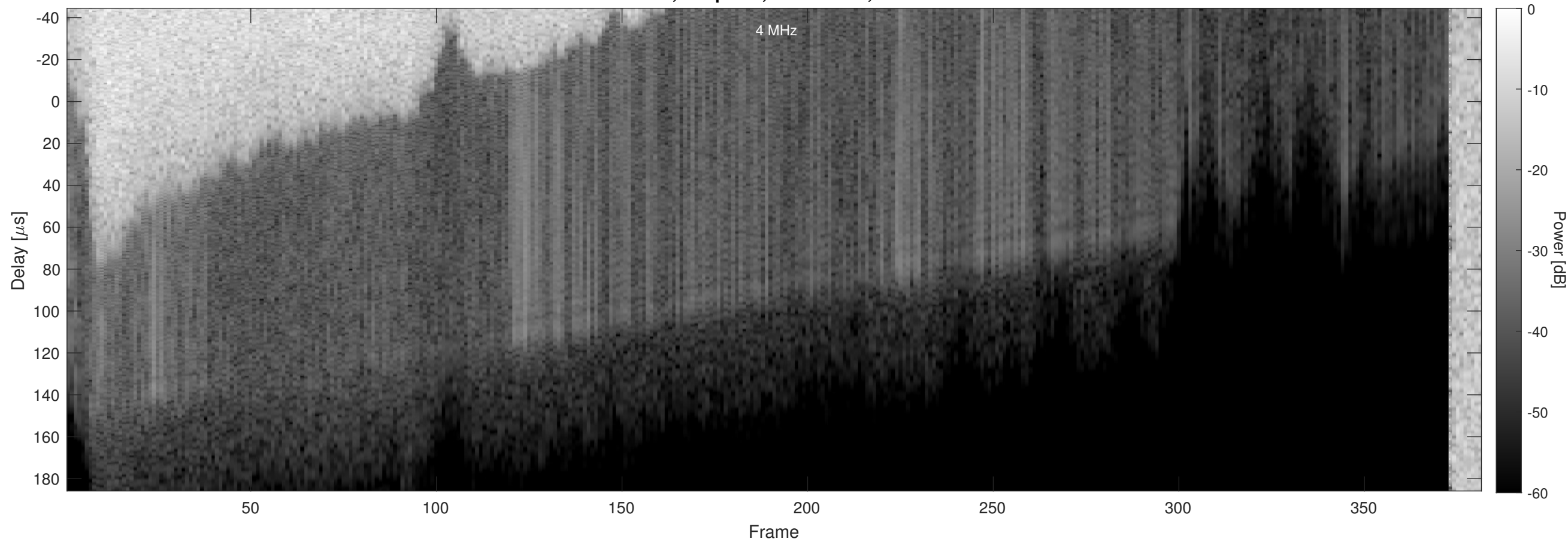
Orbit 5308, Chapman, No Window, Channel 2
