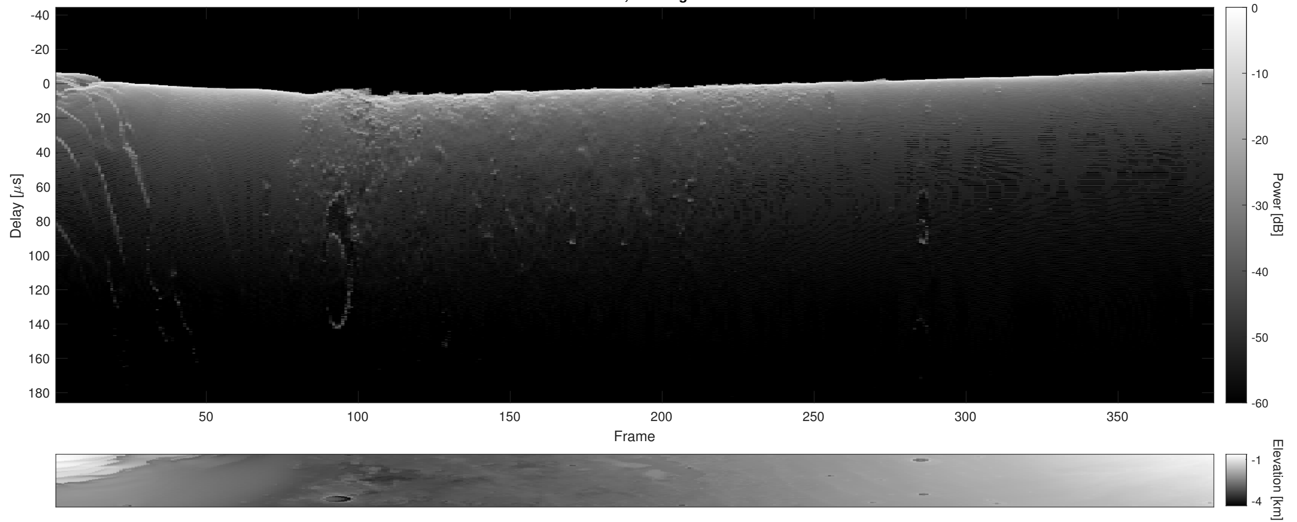
Orbit 5308, Cluttergram
