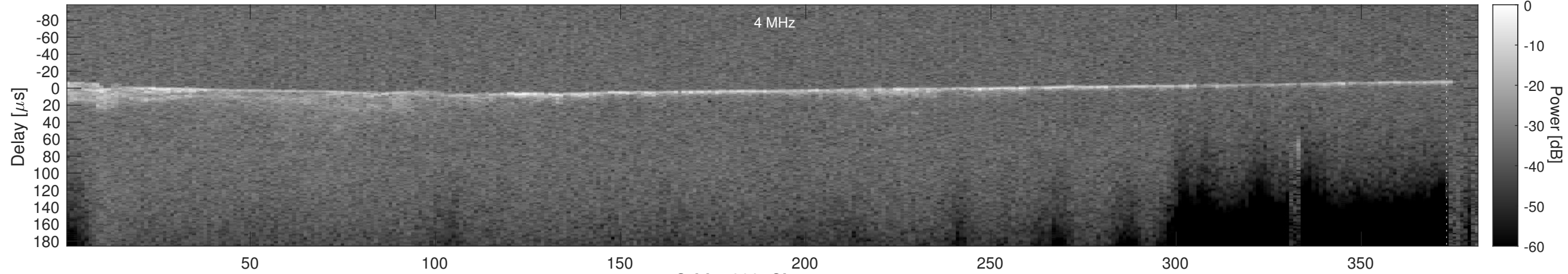
Orbit 5308, Cluttergram
