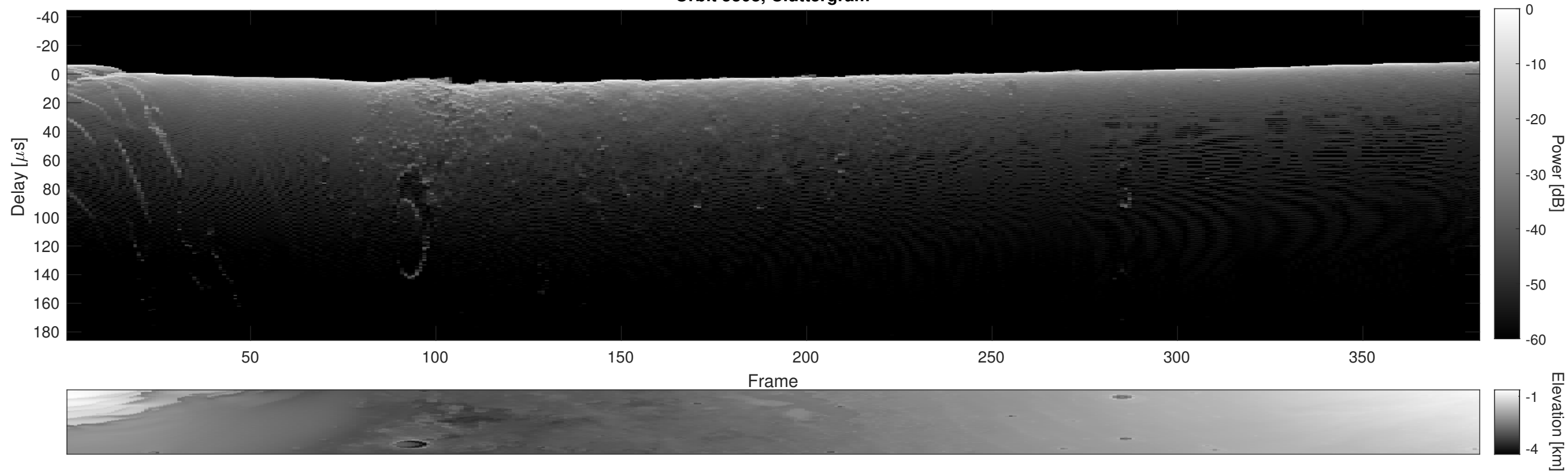
Orbit 5308, Cluttergram
